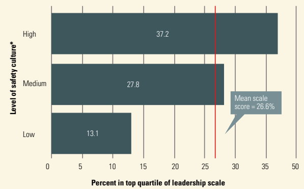
Figure 5. People leadership scale by levels of safety culture
